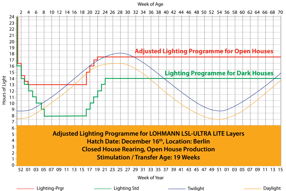
An example of a lighting programme for LOHMANN LSL-ULTRA LITE Layers adjusted to location, condition and requirements by LOHMANN TIERZUCHT lighting programme tool
